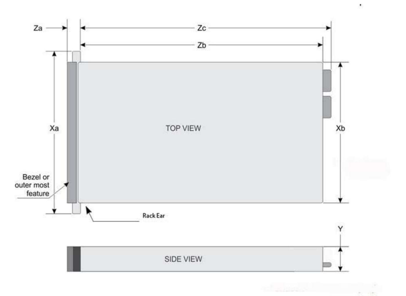
Figure 27. Chassis Dimensions for R740 and R740xd
